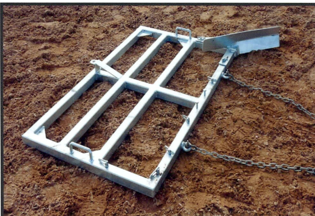
Basic Grader fitted with optional left hand Scraper
